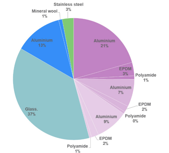
Embodied Carbon by Material (A-C) kgCO 2 eq/m 2
