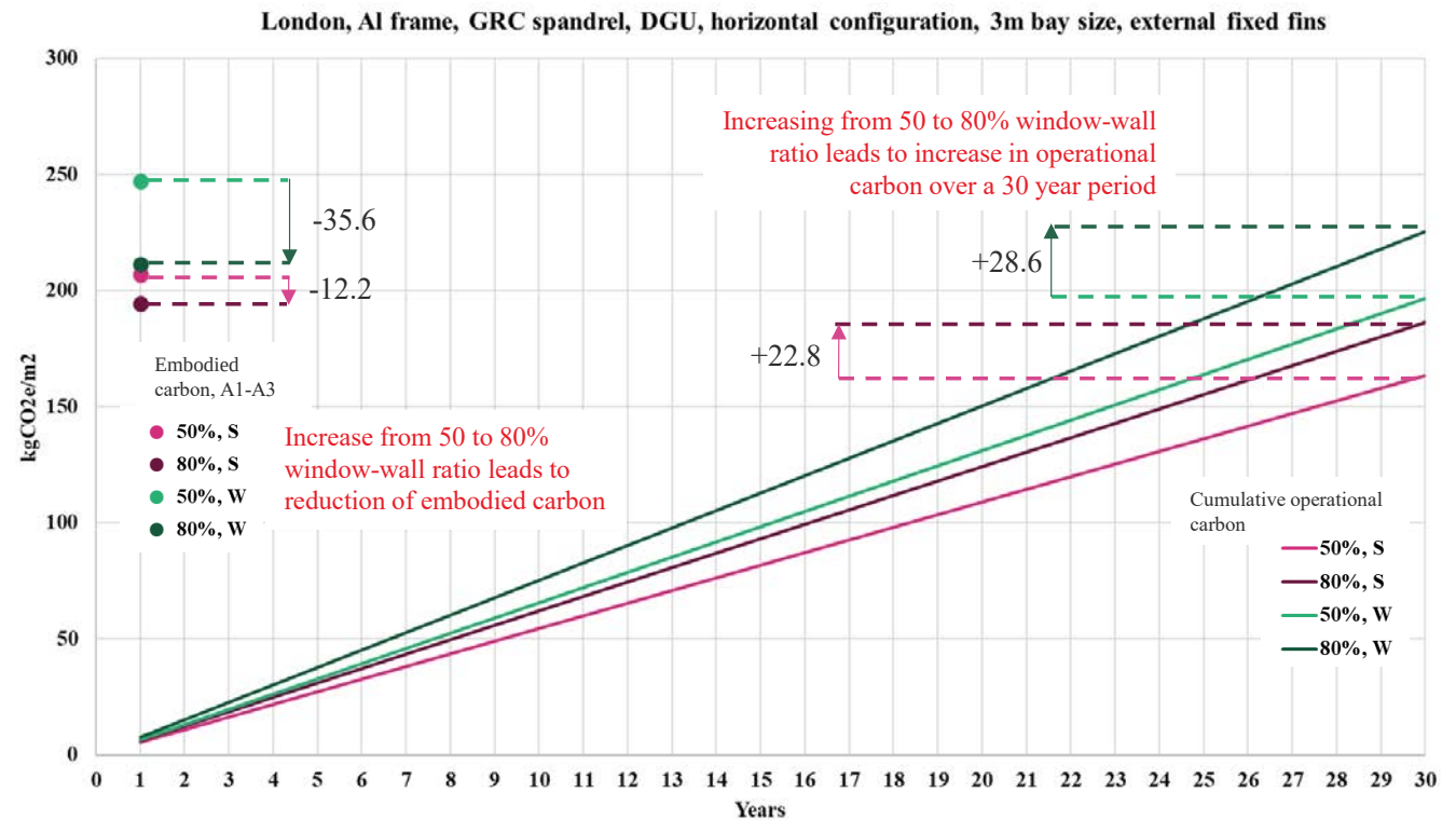
(Above) Comparing embodied gains with operational losses of increasing WWR; (Left) Graphic presentation in the variation in external fin design by changing the orientation of the façade
