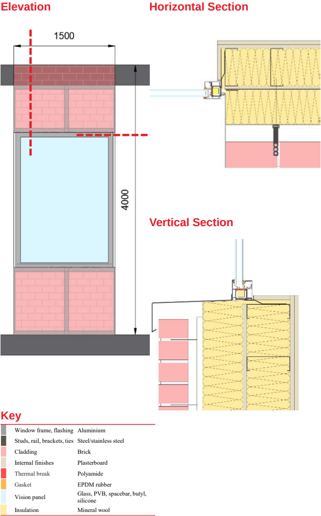
Carbon footprint of façades: significance of glass
