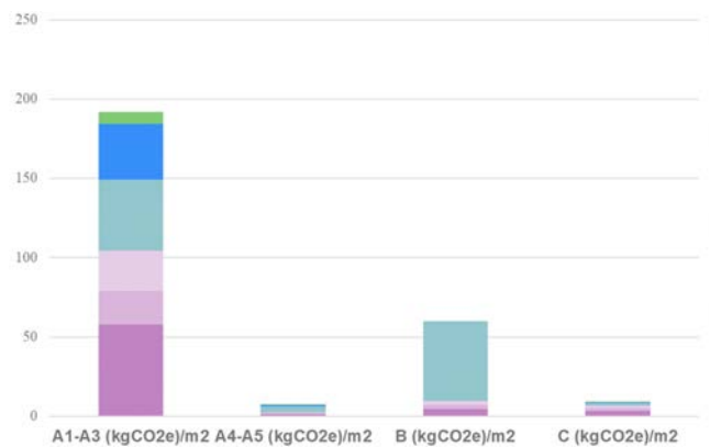
Embodied Carbon by Stage (kgCO 2 eq/m 2 )
