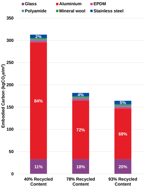
Influence of de-carbonisation of aluminium on the EC of WT-02
